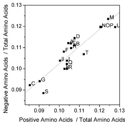
Figure 7. A plot of the number of negative amino acids divided by the total number of amino acids versus the number of positive amino acids divided by the total number of amino acids for the 20 CA isoforms listed in Table 1, identified by the label to the right of each data point. The line of best fit has a slope of 0.81 and a correlation coefficient of 0.92.
